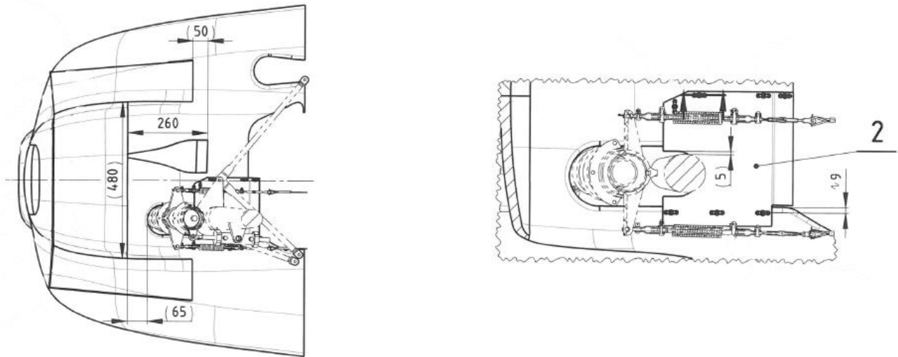
Fig. No. 2 .- Location of the cover on the aircraft (item No. 2)
